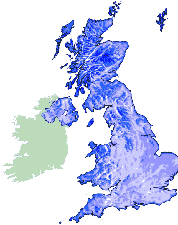
Figure 1: UK wind speed map
