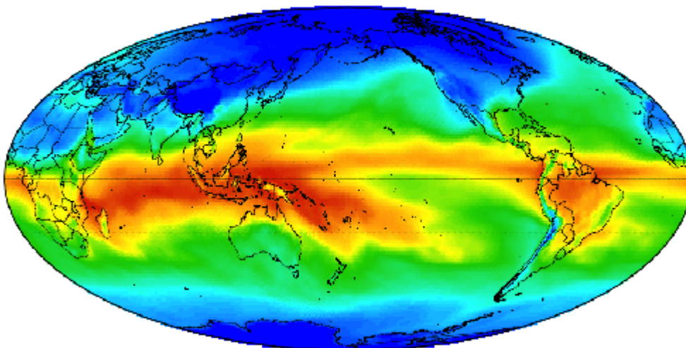
Monthly Total Precipitable Water January, 1989 Avg Globe: 22.8 NH: 18.7 SH: 26.9 Trop: 37 Arc: 2.3 Ant: 4.1 Land: 14.2 Ocean: 26.1 kg/m 2
