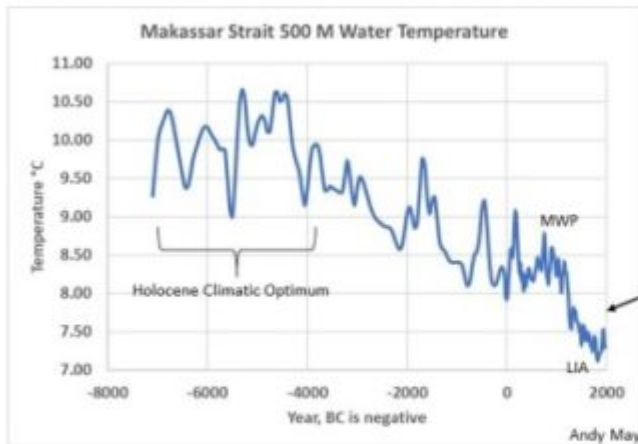
Rosenthal, et al., 2013, Science , 10,000 yr. Temperature Reconstruction of 500 m water in the Makassar Strait.
