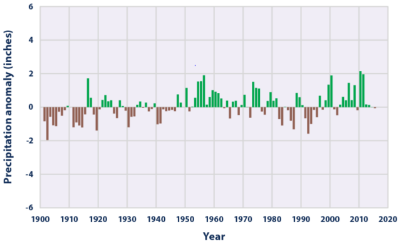
Precipitation Worldwide, 1901–2015
