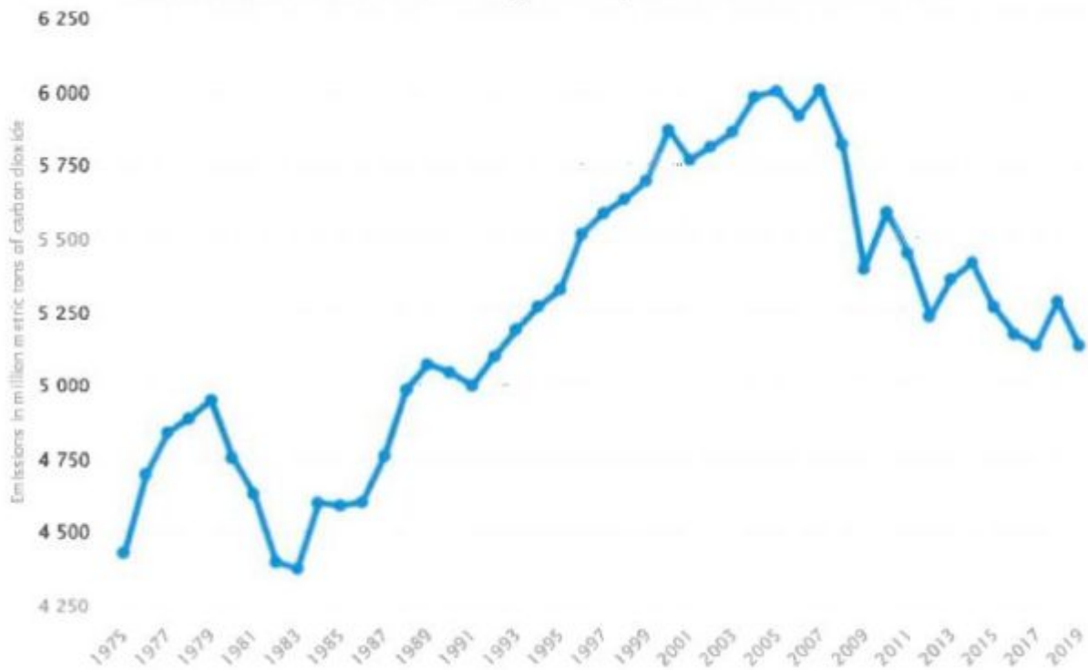
Carbon Dioxide emissions from energy consumption in the US from 1975-2020
