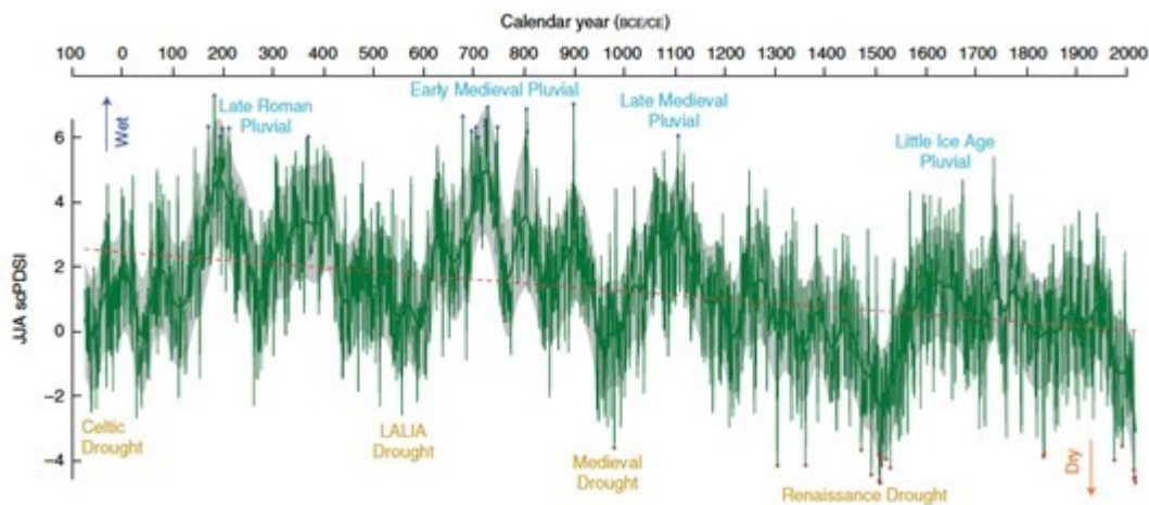
Fig. 4 | Reconstructed central European summer variability over the past 2,110 years. Reconstructed JJA scPDSI from 75 BCE to 2018 CE (Supplementary
