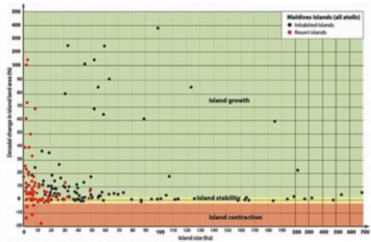
Fig. 2. Decadal change in island land area on 189 inhabited and resort islands in the Maldives. The yellow area corresponds to areal stability ( -3\% < x < 3\% ), while the green and red areas respectively indicate island expansion ( x \geq 3\% ) and contraction ( x < -3\% ). The sample islands, including islands > 100 ha, predominantly exhibited growth (108 islands; 59.3%) and secondarily experienced stability (71 islands; 38.2%). Only 5 small resort islands showed contraction.
