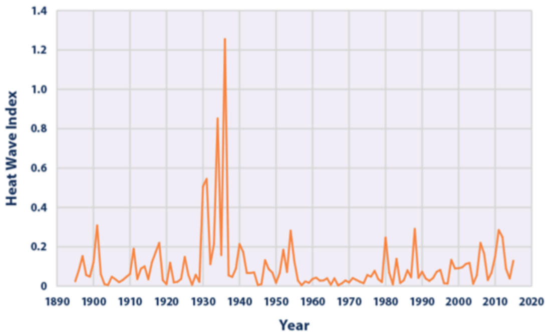
Figure 1. U.S. Annual Heat Wave Index, 1895–2015
