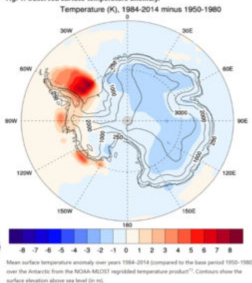
Fig. 1: Observed surface temperature anomaly.
