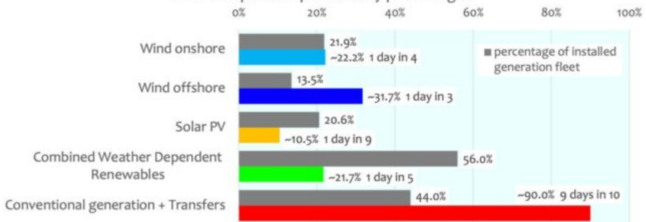
UK 2019: the proportions of electricity generation technologies and their comparative productivity percentages
