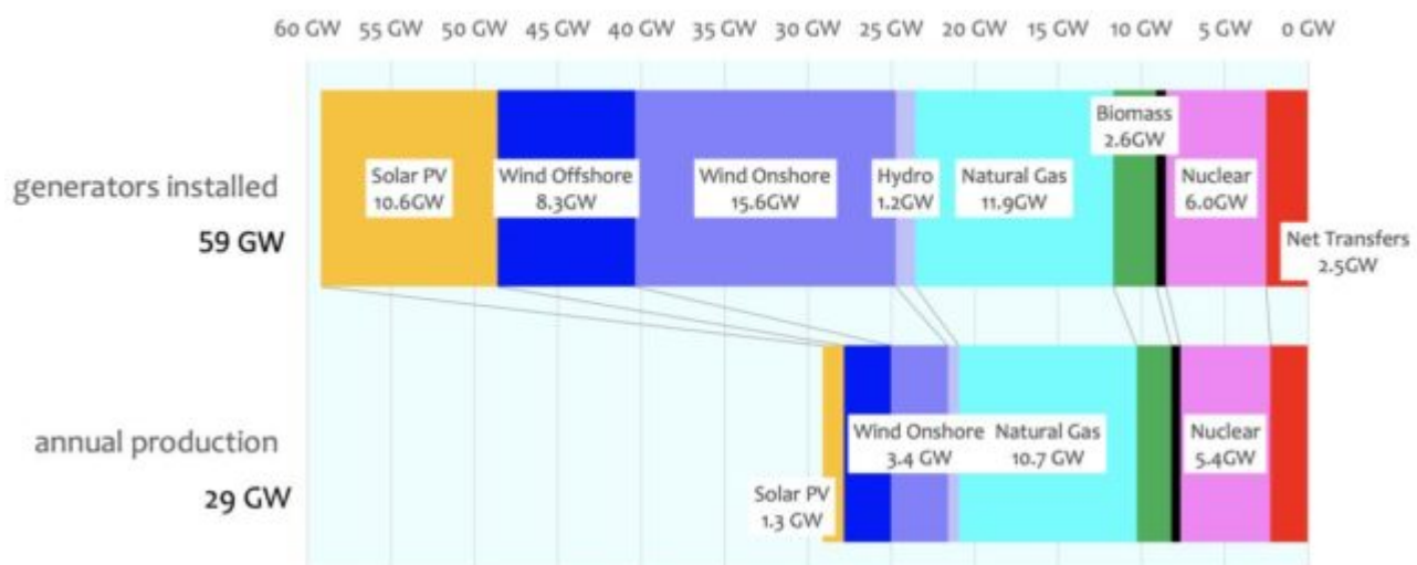
UK 2020: Generation technologies installed / annual production
