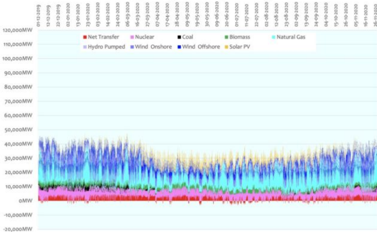
UK hourly power generation by technology: 2020
