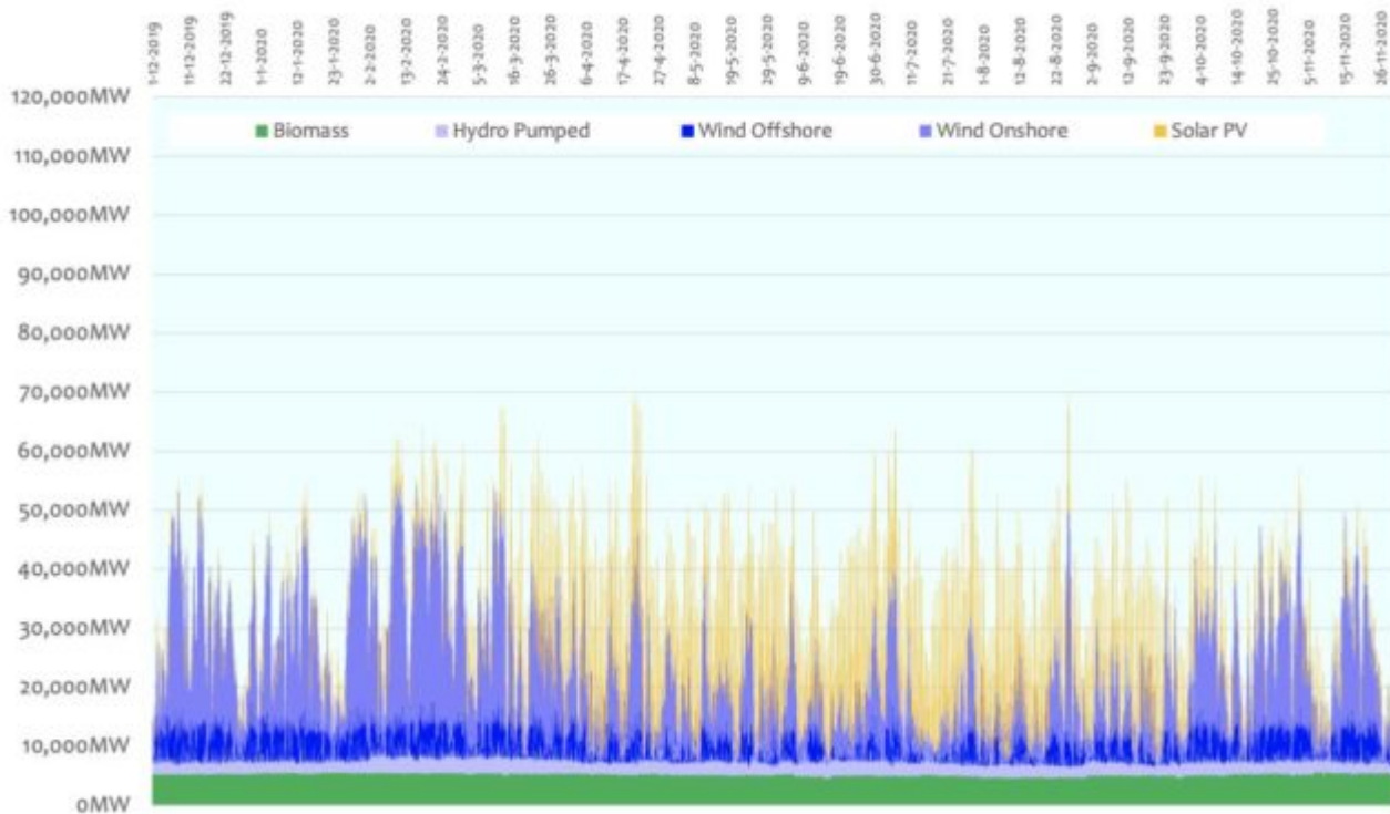
Germany hourly power output by Green technologies: 2020
