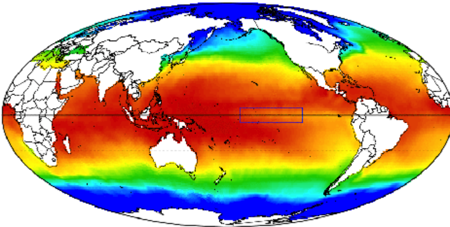
Monthly Sea Surface Temperature, Nov 1981 - Dec 2018 Reynolds Optimally Interpolated Dataset
