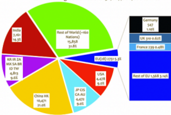
Underdeveloped world reaching the Global average CO2 4.43 tonnes/head total resulting CO2 emissions: 52,887,000,000 tonnes
