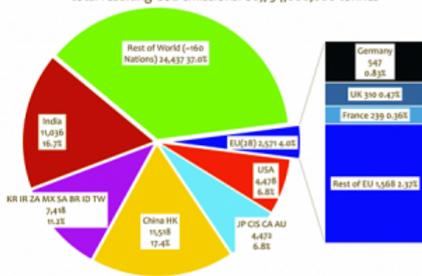
Underdeveloped world reaching the 2019 Chinese CO2 6.92 tonnes/head total resulting CO2 emissions: 68,754,000,000 tonnes
