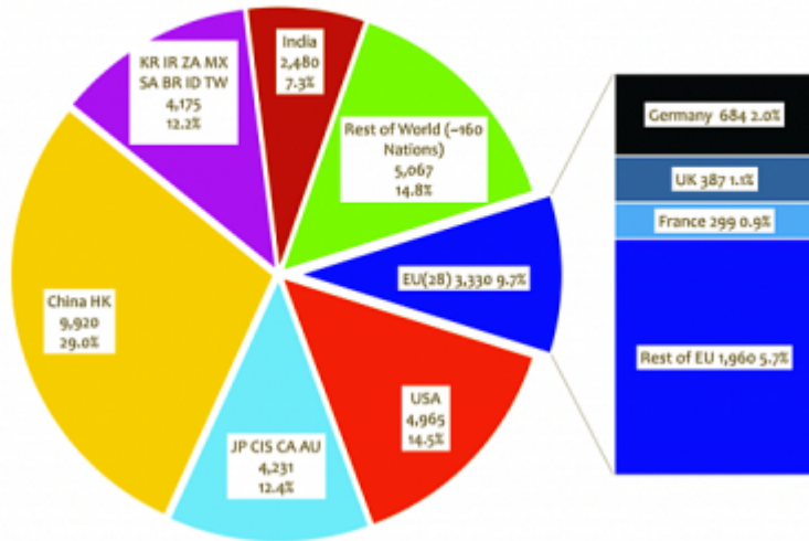
Global CO2 emissions 2019: '000,000 tonnes - percentages BPData total 2019 CO2 emissions: 34,169,000,000 tonnes
