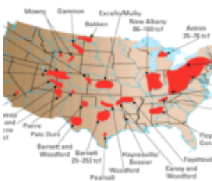
Natural Gas Shale Basins of the United States
