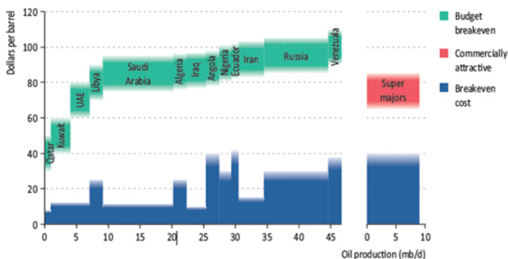
Breakeven costs, budget breakeven and commercially attractive prices for current oil production for selected producers, mid-2011
