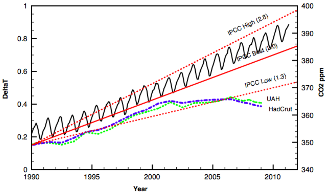
Normalised Comparison with Overlay of Moana Loa CO2 measurements
