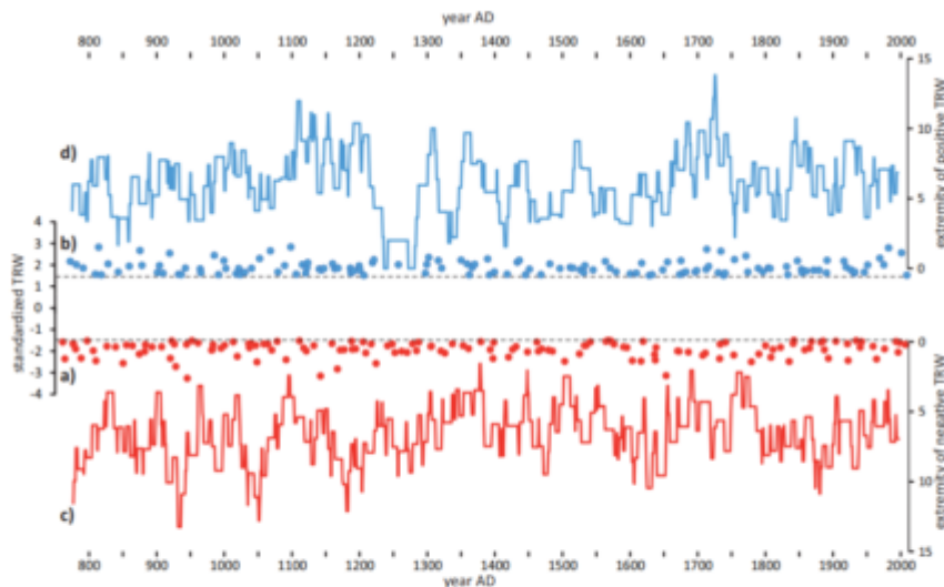
Figure 3. Negative (a) and positive (b) extremes found in the set of 18 slightly different time series of high-pass filtered TRW Czech oak chronology in the 761–2010 period; solid lines represent extremity index of negative (c) and positive (d) years calculated for a 30-year moving window (see text for details of extremity index).
