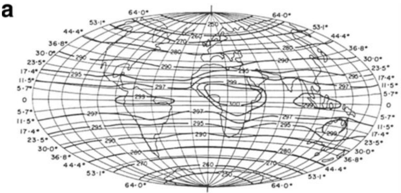
Abbildung 4: “Global distribution[s] of (a) mean air temperature, ..., predicted with the constraint of maximum entropy production (equation (9)). Reprinted from Paltridge [1978]” aus Ozawa et al. (2003, Figure 4)
