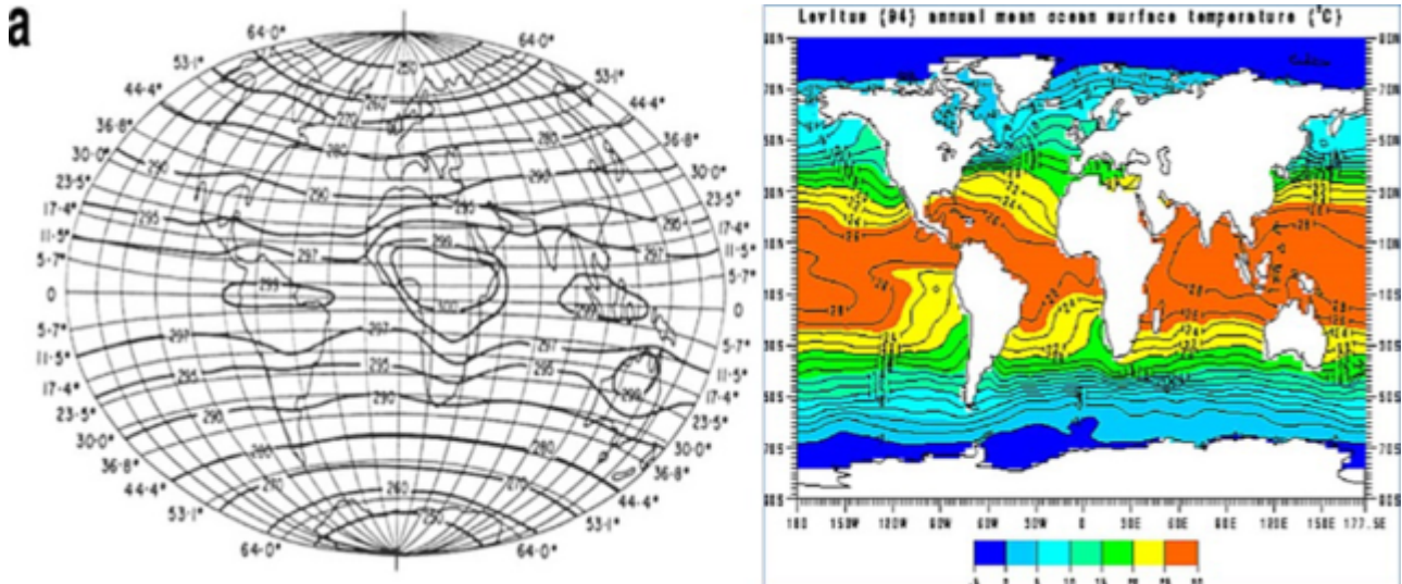
Abbildung 5: Globale Durchschnittstemperaturen (Abbildungen in E-W-Richtung gestaucht) Links: Paltridge [1978] aus Ozawa et al. (2003, Figure 4) "Global distribution[s] of (a) mean air temperature, ..., predicted with the constraint of maximum entropy production (equation (9))." Rechts: NASA "Annual Mean Ocean Surface Temperature" based on observed data up until 1994
