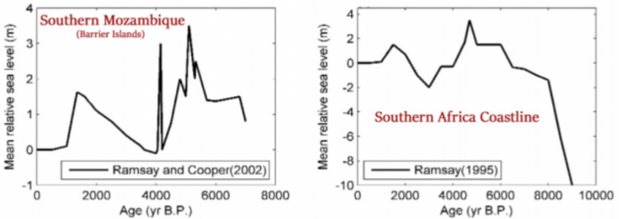
Fig. 2. Relative sea level curves for the Mozambique coastline, southeastern Africa.
