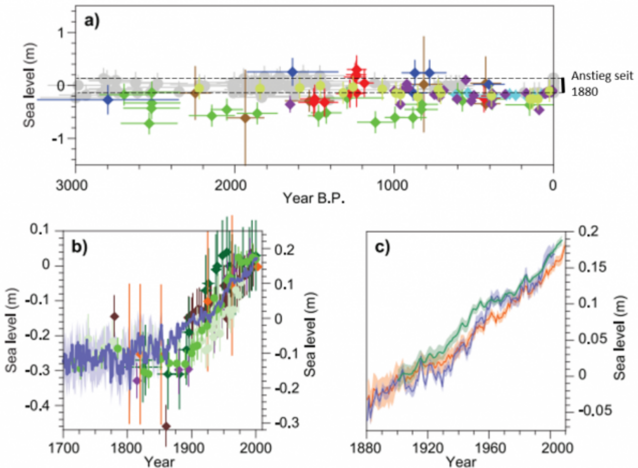
Bild 8 Pegelgrafiken (Anm.: Vom Autor ergänzt) [6] AR5 (Teilbild) Zu der Abbildung: Figure 13.3 | (a) Paleo sea level data for the last 3000 years from Northern and Southern Hemisphere sites. The effects of glacial isostatic adjustment (GIA) have been removed from these records. Light green = Iceland (Gehrels et al., 2006), purple = Nova Scotia (Gehrels et al., 2005), bright blue = Connecticut (Donnelly et al., 2004), blue = Nova Scotia (Gehrels et al., 2005), red = United Kingdom (Gehrels et al., 2011), green = North Carolina (Kemp et al., 2011), brown = New Zealand (Gehrels et al., 2008), grey = mid-Pacific Ocean (Woodroffe et al., 2012) (b) Paleo sea level data from salt marshes since 1700 from Northern and Southern Hemisphere sites compared to sea level reconstruction from tide gauges (blue time series with uncertainty) (Jevrejeva et al., 2008). The effects of GIA have been removed from these records by subtracting the long-term trend (Gehrels and Woodworth, 2013). Ordinate axis on the left corresponds to the paleo sea level data. Ordinate axis on the right corresponds to tide gauge data. Green and light green = North Carolina (Kemp et al., 2011), orange = Iceland (Gehrels et al., 2006), purple = New Zealand (Gehrels et al., 2008), dark green = Tasmania
