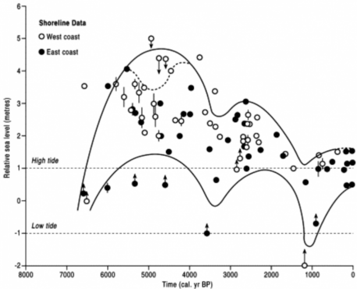
Bild 19 Fig. 7. Holocene sea-level envelope for Peninsula Malaysia (modified from Tija, 1996). Data points with arrows indicate directional (limiting) index points. Some index points have vertical error bars, where the vertical range of the sea-level indicator is understood. No
