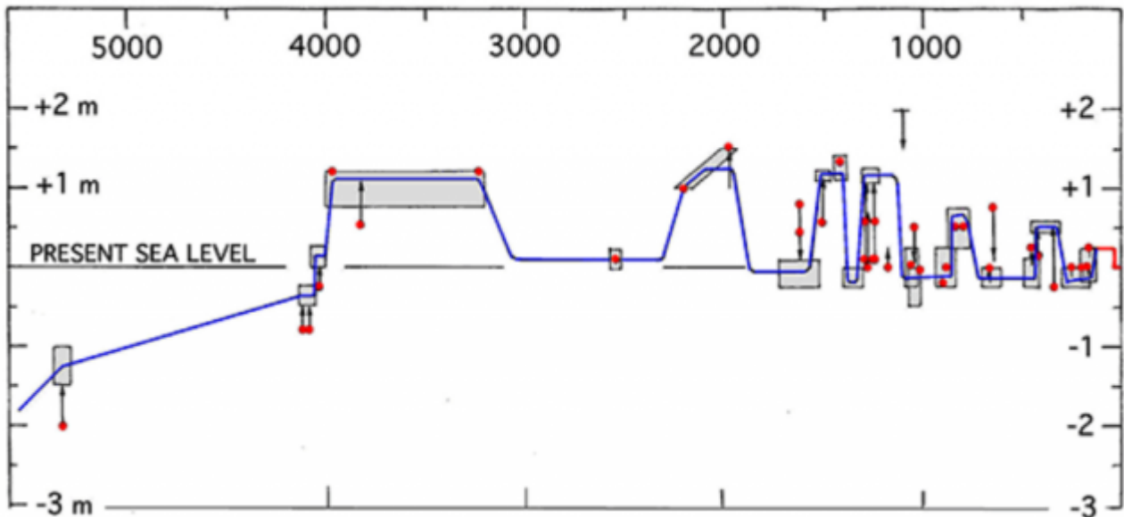
Bild 21 Fig. 2. The Late Holocene sea level changes in the Maldives (Mörner, 2007) including 7 transgression peaks in the last 4000 years with 3 peaks in the last millennium.
