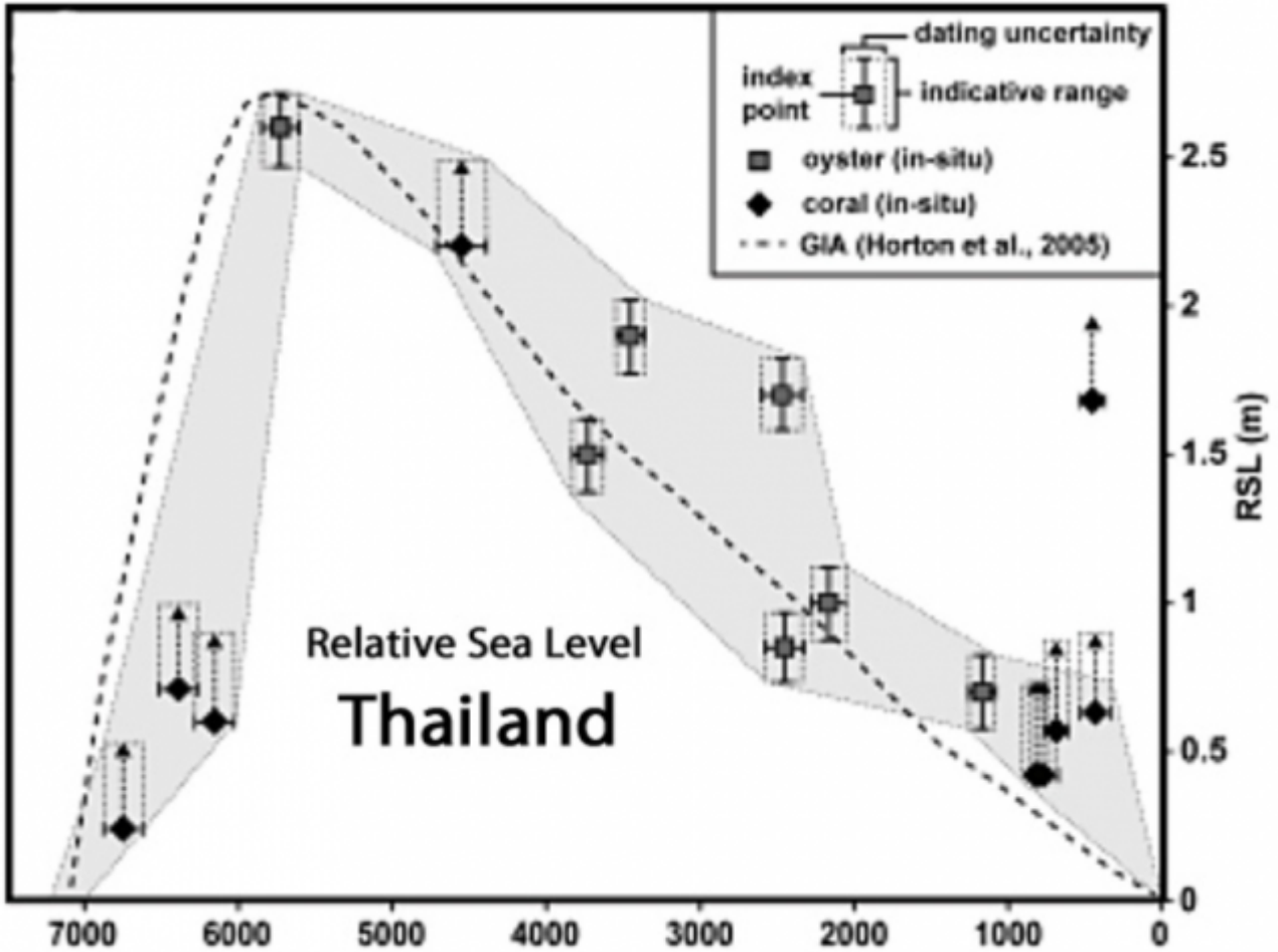
Bild 10a Anja Scheffers, Dominik Brill, Dieter Kelletat, April 11, 2012: Holocene sea levels along the Andaman Sea coast of Thailand
