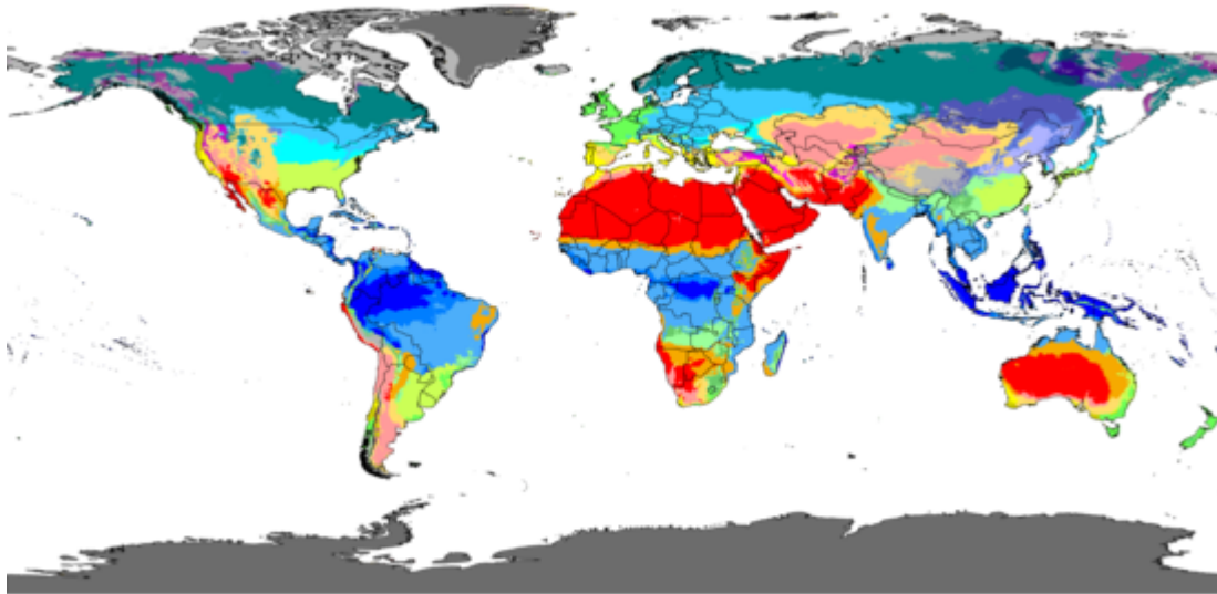
Köppen-Geiger climate classification map (1980-2016)
