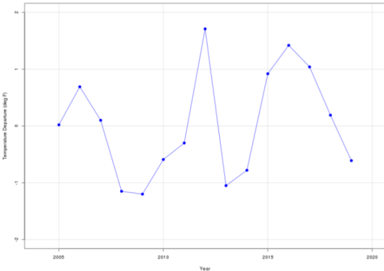
2005 - 2019, USA48 Temperature Departure from Climatology
