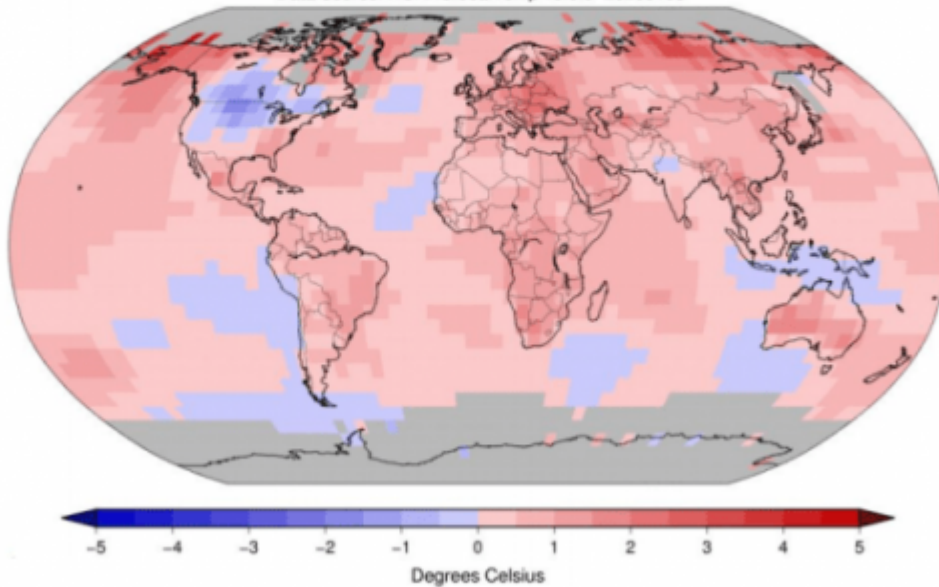
Land & Ocean Temperature Departure from Average Jan–Dec 2019 (with respect to a 1981–2010 base period)
