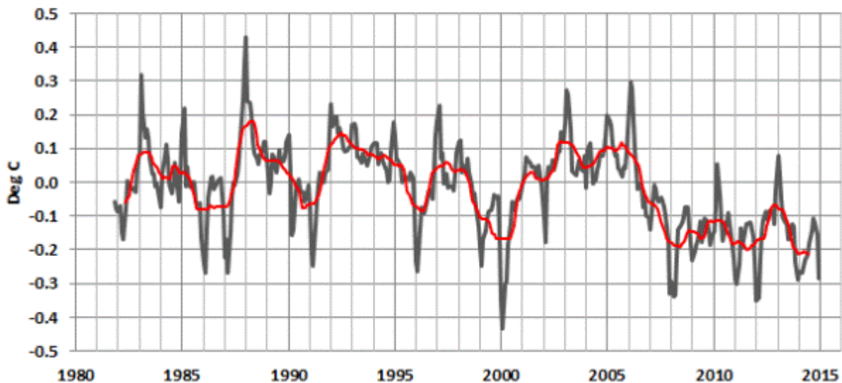
Southern Ocean Sea Surface Temperature Anomalies (Reynolds OI.v2 through KNMI Climate Explorer) Smoothed w/ 13-Month Running-Mean Filter Nov 1981 to Dec 2014 Change: Dec 2014 Minus Nov 2014 = -0.128 Deg C
