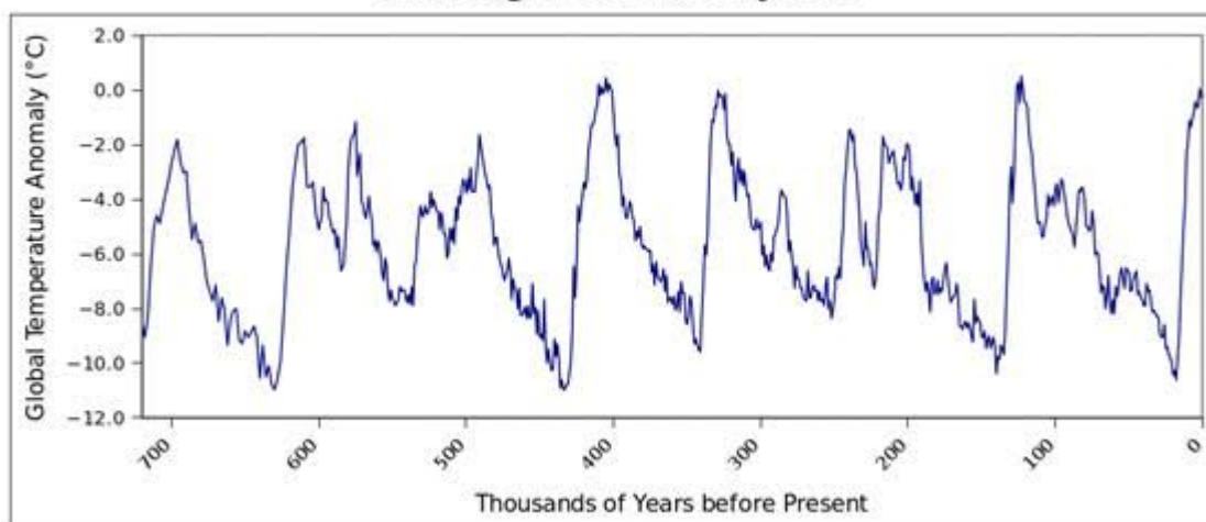
Last Eight Climate Cycles
