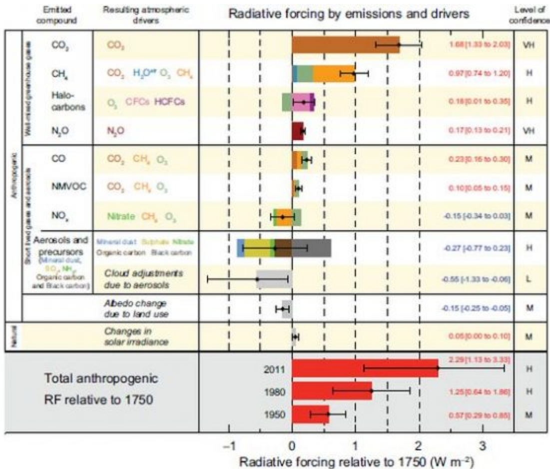
Figure SP.M.5 | Radiative forcing estimates in 2011 relative to 1750 and aggregated uncertainties for the main drivers of climate change. Values are global average radiative forcing (RF 16 ), partitioned according to the emitted compounds or processes that result in a combination of drivers. The best estimates of the net radiative forcing are shown as black diamonds with corresponding uncertainty intervals; the numerical values are provided on the right of the figure, together with the confidence level in the net forcing (VH – very high, H – high, M – medium, L – low, VL – very low). Albedo forcing due to black carbon on snow and ice is included in the black carbon aerosol bar. Small forcings due to contrails (0.05 W m -2 , including contrail induced cirrus), and HFCs, PFCs and SF 2 (total 0.03 W m -2 ) are not shown. Concentration-based RFs for gases can be obtained by summing the like-coloured bars. Volcanic forcing is not included as its episodic nature makes it difficult to compare to other forcing mechanisms. Total anthropogenic radiative forcing is provided for three different years relative to 1750. For further technical details, including uncertainty ranges associated with individual components and processes, see the Technical Summary Supplementary Material. (8.5; Figures 8.14–8.18; Figures TS.6 and TS.7)
