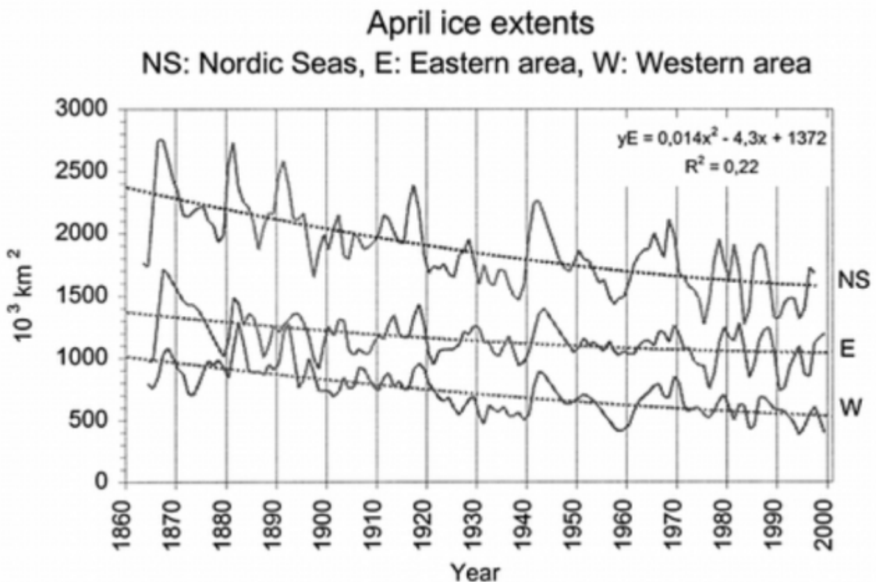
Bild 3-8 [23] MartinJakobsson et al., 2010: New insights on Arctic Quaternary climate
