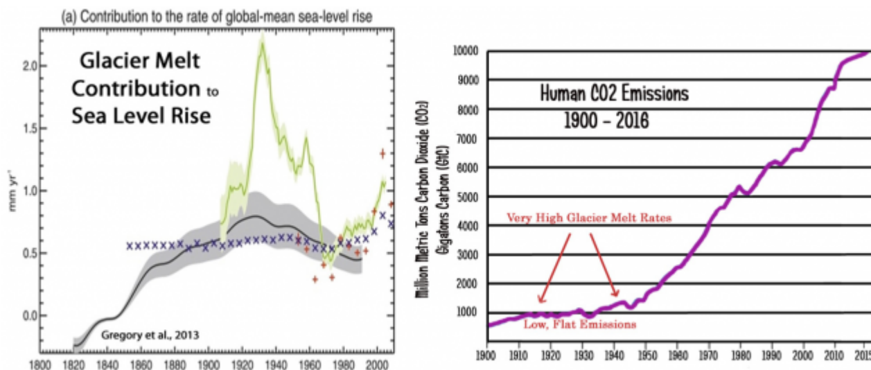
Bild 3-5 Globally, glaciers melted 69% more rapidly from 1921-1960 (12.5 meters/year) than from 1961-2000 (7.4 meters/year).
