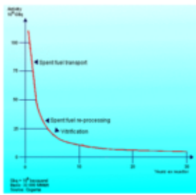
Change in radioactivity of fission products – one tonne of spent PWR fuel
