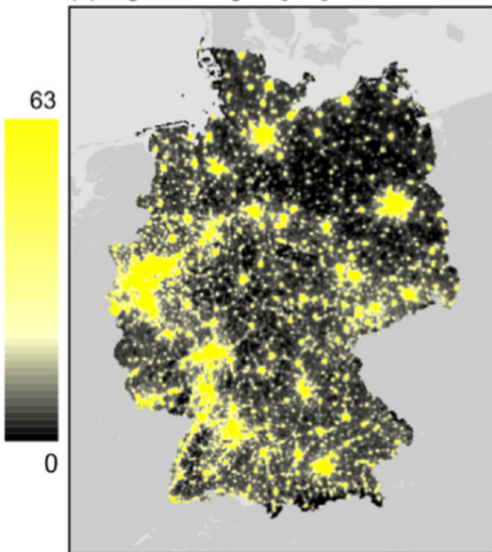
(a) Night-time lights [DN]
