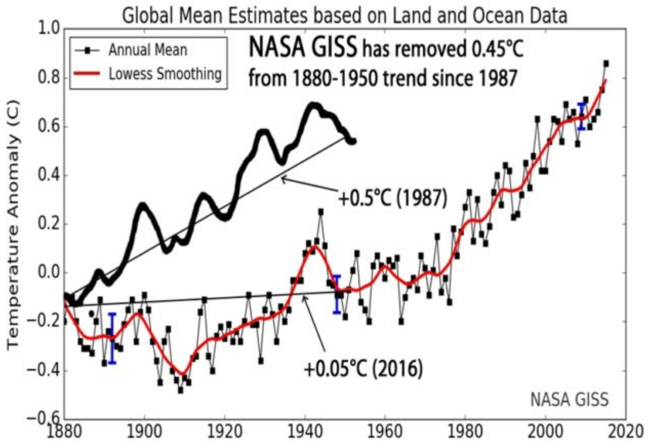
NASA GISS graph
