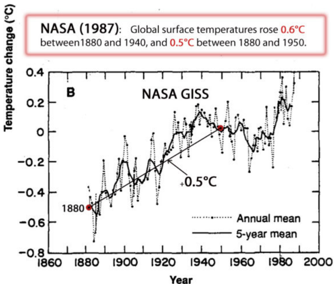
Fig. 2. A comparison of the global surface temperature trends of the past 100 years constructed from land and island stations and ocean surface temperature data sets at the (A) Climatic Research Unit and from a similar set of stations (minus the ocean surface temperature data set) at the (B) Goddard Institute for Space Studies.
