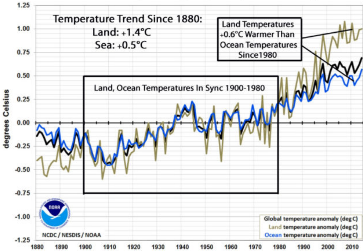
NOAA Global Land vs. Sea
