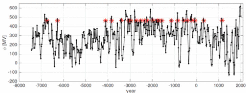
Figure 20. Modulation potential record \Phi [MV] used for forecasting solar activity. What matters is the relative variation in \Phi , which reflects that in the TSE large values of \Phi correspond to grand solar maxima, whereas low values correspond to grand solar minima. Red stars refer to the events used in the analogue forecast, see Sec. 3.1.1.
