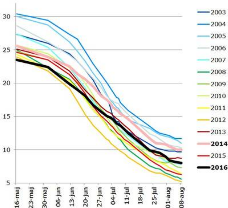
Arctic sea ice volume estimated from DMI online graphs. Unit: 1000 km 3 Arctic sea ice
