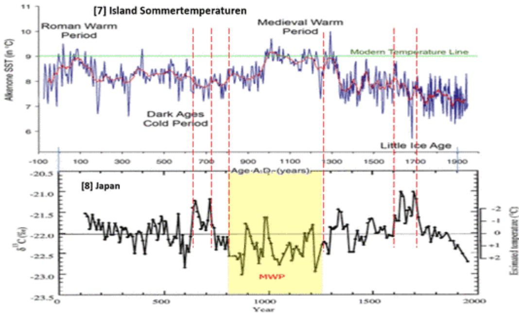
A 2000-Year Summer Sea Surface Temperature Record derived from an Ocean Sediment Core off the Coast of North Iceland (Adapted from Sicre et al. 2008)
