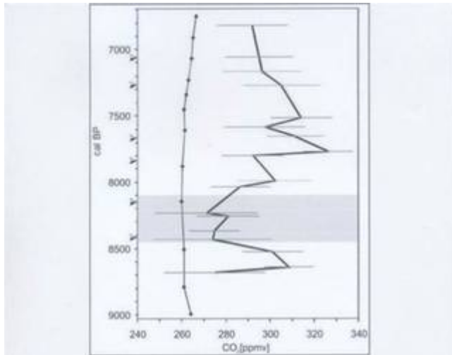
Fig 2. Reconstructed CO 2 concentrations for the time interval between ≈8,700 and ≈6,800 calendar years B.P. based on CO 2 extracted from air in Antarctic ice of Taylor Dome (left curve; ref. 2; raw data available via www.ngdc.noaa.gov/paleo/ky/taylor.html ) and SI data for fossil B. pendula and B. pubescens from Lake Lille Gribst, Denmark (right curve; see Table 1). The arrows indicate accelerator mass spectrometry 14 C chronologies used for temporal control (Table 1). The shaded time interval corresponds to the 8.2-ka-B.P. cooling event (3–12). Quantification of mean CO 2 concentrations is based on the rate of historical CO 2 responsiveness of the European tree birches (Fig. 1); ±1σ CO 2 estimates are derived from the standard deviation of the SI mean values. Proc Natl Acad Sci U S A. 2002 September 17; 99(19): 12011–12014.
