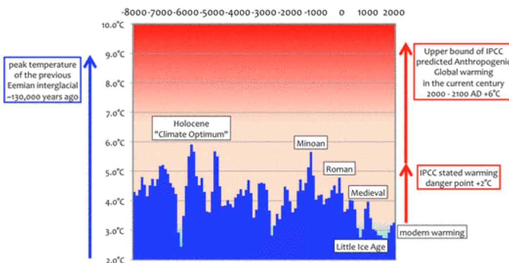
GRIP Ice Core data progress of the current Holocene epoch: compared to the previous interglacial Eemian temperature peak and the prediction of Catastrophic Global Warming Alarmists for the coming century
