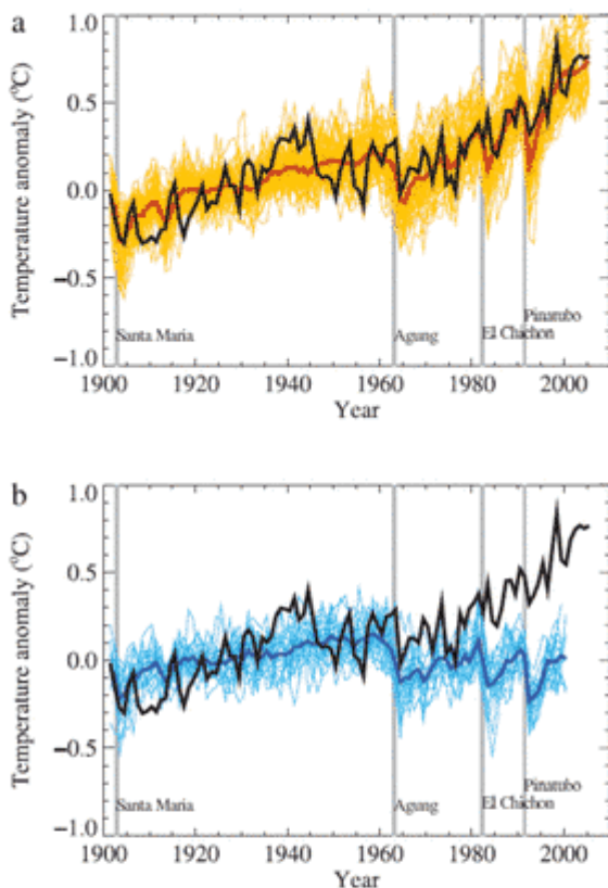
Figure 9.5. Comparison between global mean surface temperature anomalies ( ^{\circ}\text{C} ) from observations (black) and AOGCM simulations forced with (a) both anthropogenic and natural forcings and (b) natural forcings only. All data are shown as global mean temperature anomalies relative to the period 1901 to 1950, as observed (black, Hadley Centre/Climatic Research Unit gridded surface temperature data set (HadCRUT3); Brohan et al., 2006) and, in (a) as obtained from 58 simulations produced by 14 models with both anthropogenic and natural forcings. The multi-model ensemble mean is shown as a thick red curve and individual simulations are shown as thin yellow curves. Vertical grey lines indicate the timing of major volcanic events. Those simulations that ended before 2005 were extended to 2005 by using the first few years of the IPCC Special Report on Emission Scenarios (SRES) A1B scenario simulations that continued from the respective 20th-century simulations, where available. The simulated global mean temperature anomalies in (b) are from 19 simulations produced by five models with natural forcings only. The multi-model ensemble mean is shown as a thick blue curve and individual simulations are shown as thin blue curves. Simulations are selected that do not exhibit excessive drift in their control simulations (no more than 0.2^{\circ}\text{C} per century). Each simulation was sampled so that coverage corresponds to that of the observations. Further details of the models included and the methodology for producing this figure are given in the Supplementary Material, Appendix 9.C. After Stott et al. (2006b).
