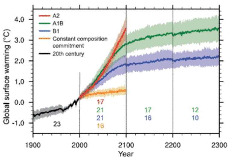
Figure 10.4. Multi-model means of surface warming (relative to 1980–1999) for the scenarios A2, A1B and B1, shown as continuations of the 20th-century simulation. Values beyond 2100 are for the stabilisation scenarios (see Section 10.7). Linear trends from the corresponding control runs have been removed from these time series. Lines show the multi-model means, shading denotes the \pm 1 standard deviation range of individual model annual means. Discontinuities between different periods have no physical meaning and are caused by the fact that the number of models that have run a given scenario is different for each period and scenario, as indicated by the coloured numbers given for each period and scenario at the bottom of the panel. For the same reason, uncertainty across scenarios should not be interpreted from this figure (see Section 10.5.4.6 for uncertainty estimates).
