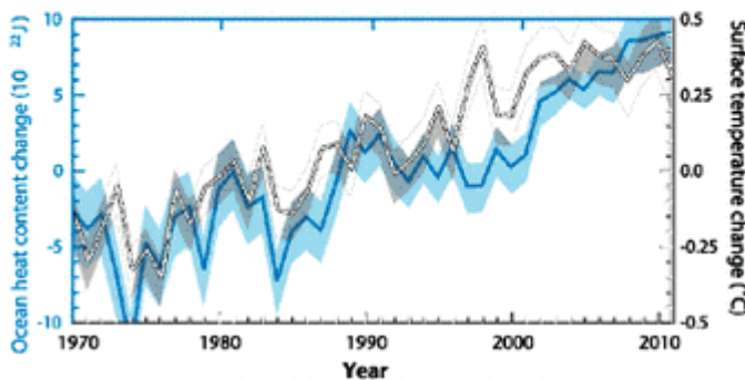
Two Different Presentations of Unidentified Ocean Heat Content Datasets from 2013 UKMO Report
